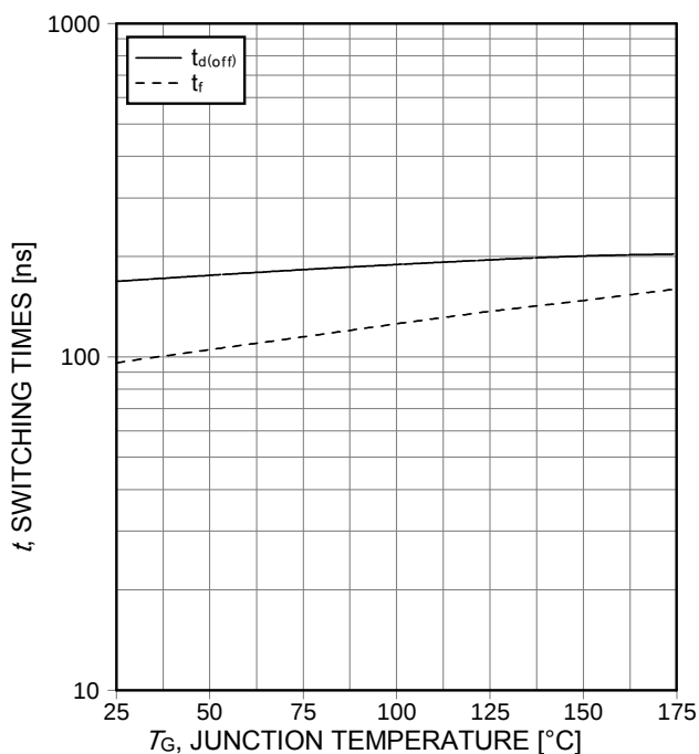
Figure 11. Typical switching times as a function of junction temperature (inductive load, V_{CE}=400\text{V} , V_{GE}=15/0\text{V} , I_C=10\text{A} , R_G=23\Omega , Dynamic test circuit in Figure E)
