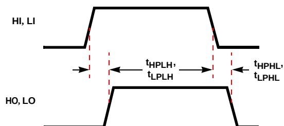
FIGURE 3. PROPAGATION DELAYS
