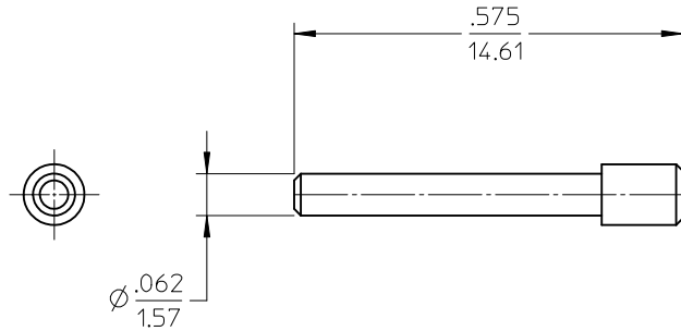
MATERIAL NO. 845090001 CONTACT SIZE 20
