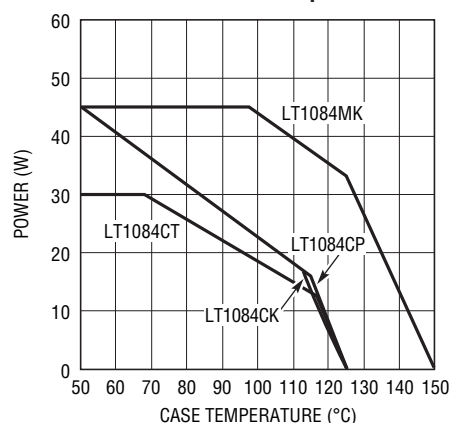
LT1084 Maximum Power Dissipation*
