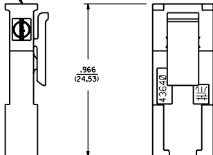
MATED MICRO-FIT CONNECTOR
