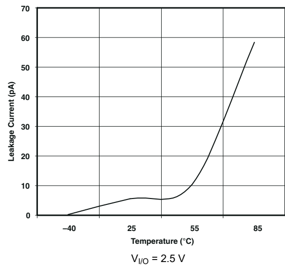
Figure 6-2. Leakage Current vs Temperature
