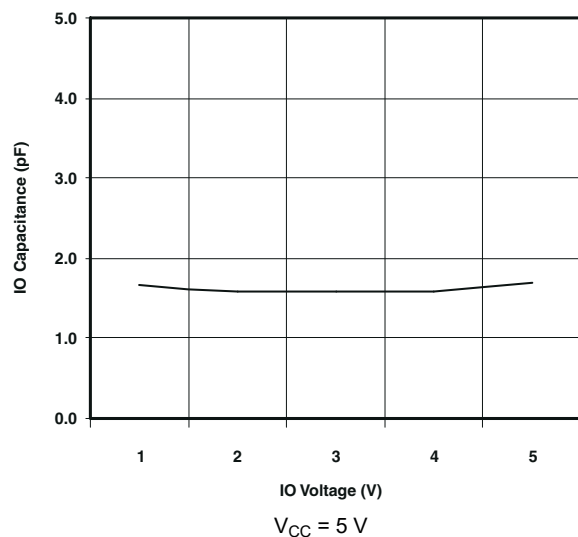
Figure 6-4. I/O Capacitance vs Input Voltage
