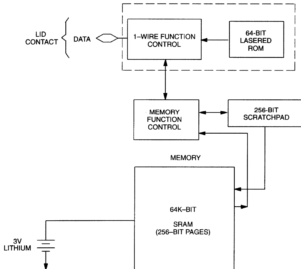
DS1996 BLOCK DIAGRAM Figure 1
