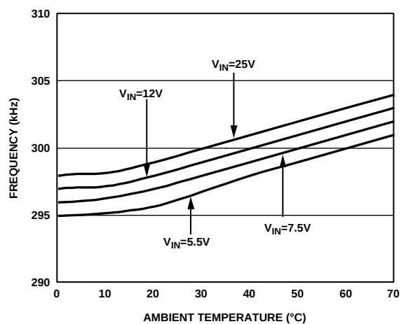
Figure 9. Oscillator Frequency vs. Temperature
