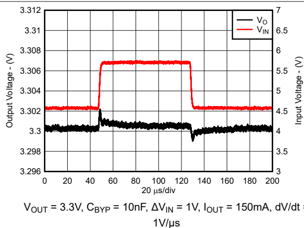
Figure 5-50. Line Transient Response (New Chip)
