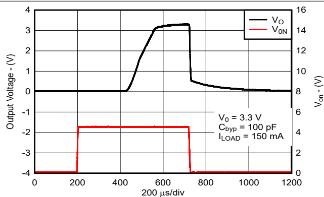
Figure 5-52. Turn-On Time (New Chip)
