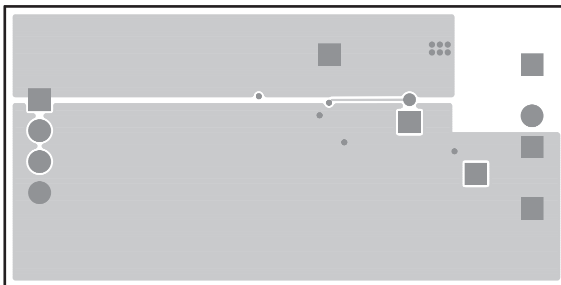
Figure 3. Bottom Layer
