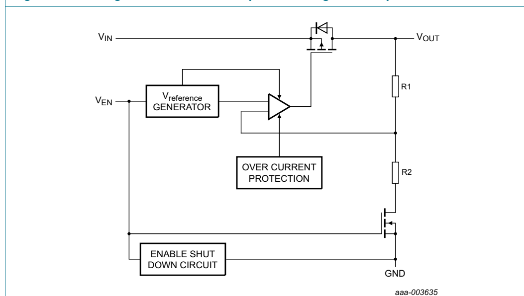
Fig 3. Block diagram of LD6815TD/xxH
