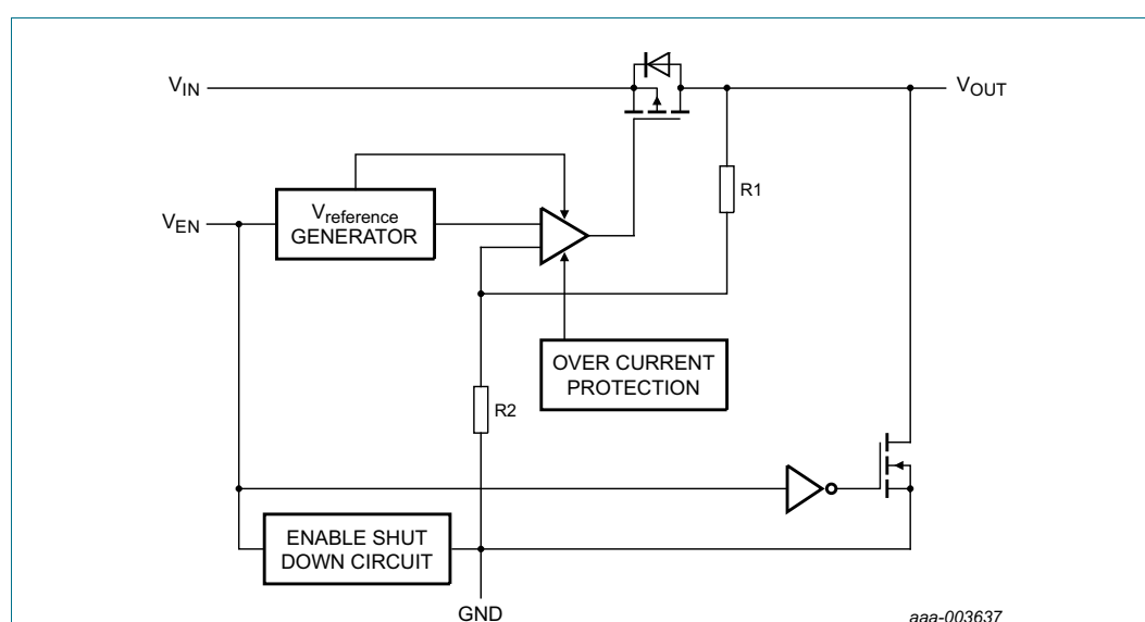
Fig 2. Block diagram of LD6815TD/xxP (auto discharge function)
