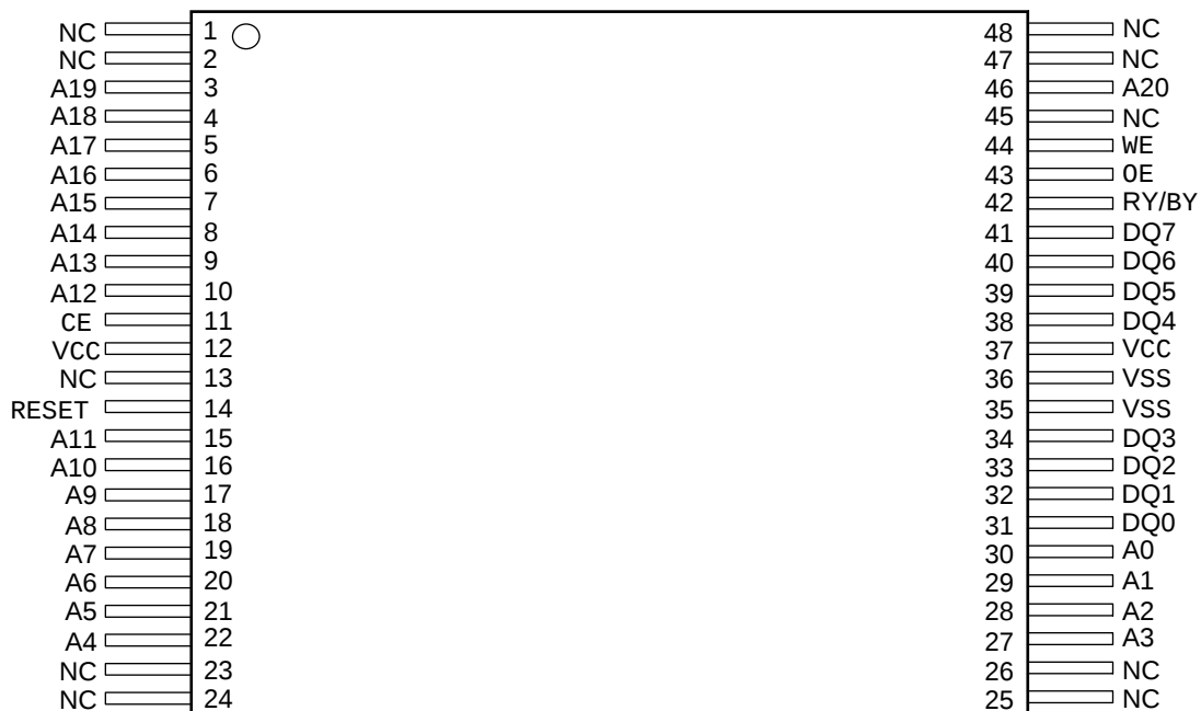
Standard TSOP
