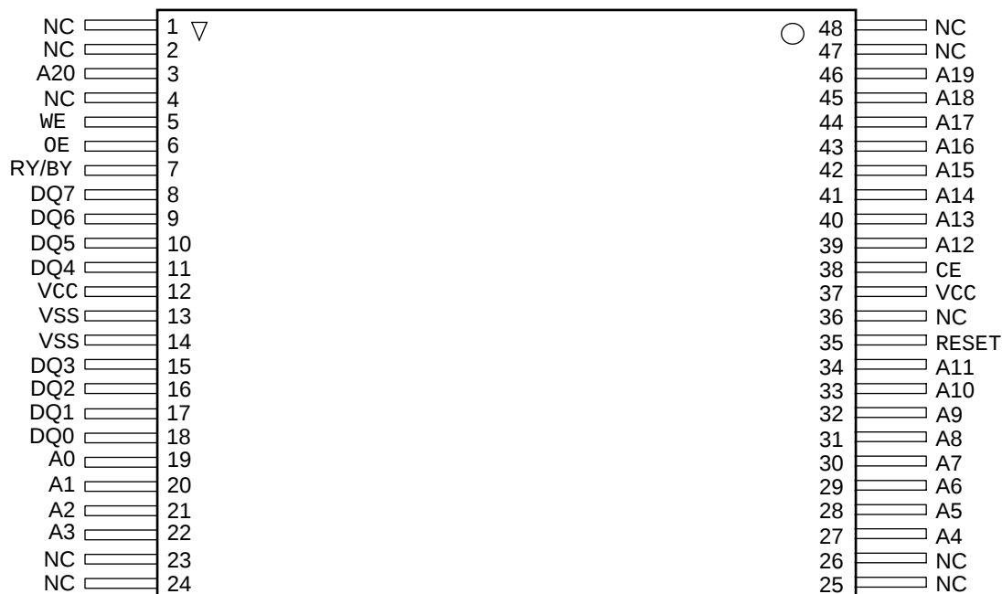
Reverse TSOP
