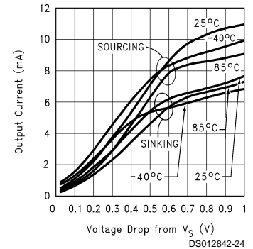
V_O vs I_O , V_S = \pm 1.1\text{V}
