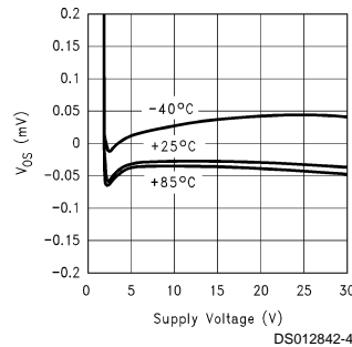
V_{\text{OS}} vs Supply Voltage
