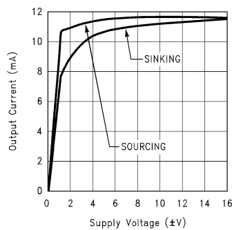
Short Circuit Current vs Supply Voltage
