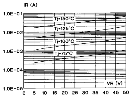
Fig. 8 : Reverse leakage current versus reverse voltage applied. (Typical values)
