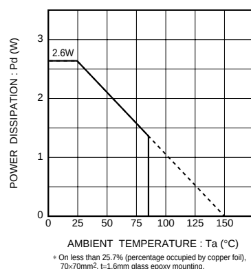
Fig.4 Power dissipation
