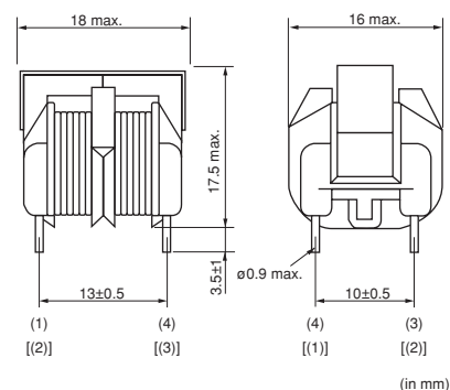
Standard Winding
