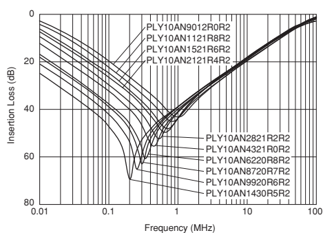
Standard Winding
