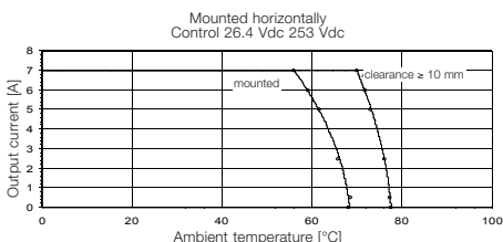
WRS 2 115 VUC/230 VAC • 8418290000
