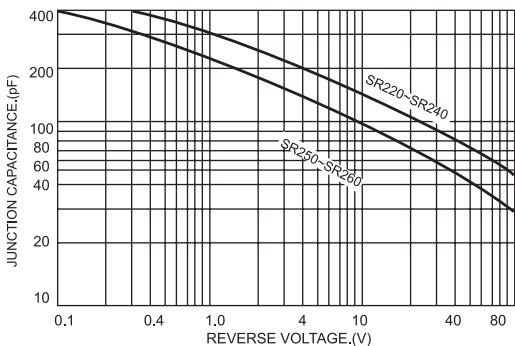
FIG.4-TYPICAL JUNCTION CAPACITANCE
