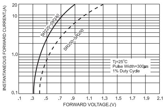
FIG.2-TYPICAL FORWARD CHARACTERISTICS
