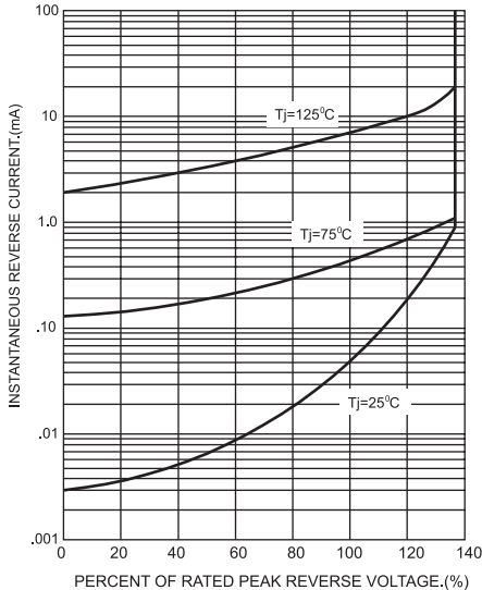
FIG.3-TYPICAL REVERSE CHARACTERISTICS
