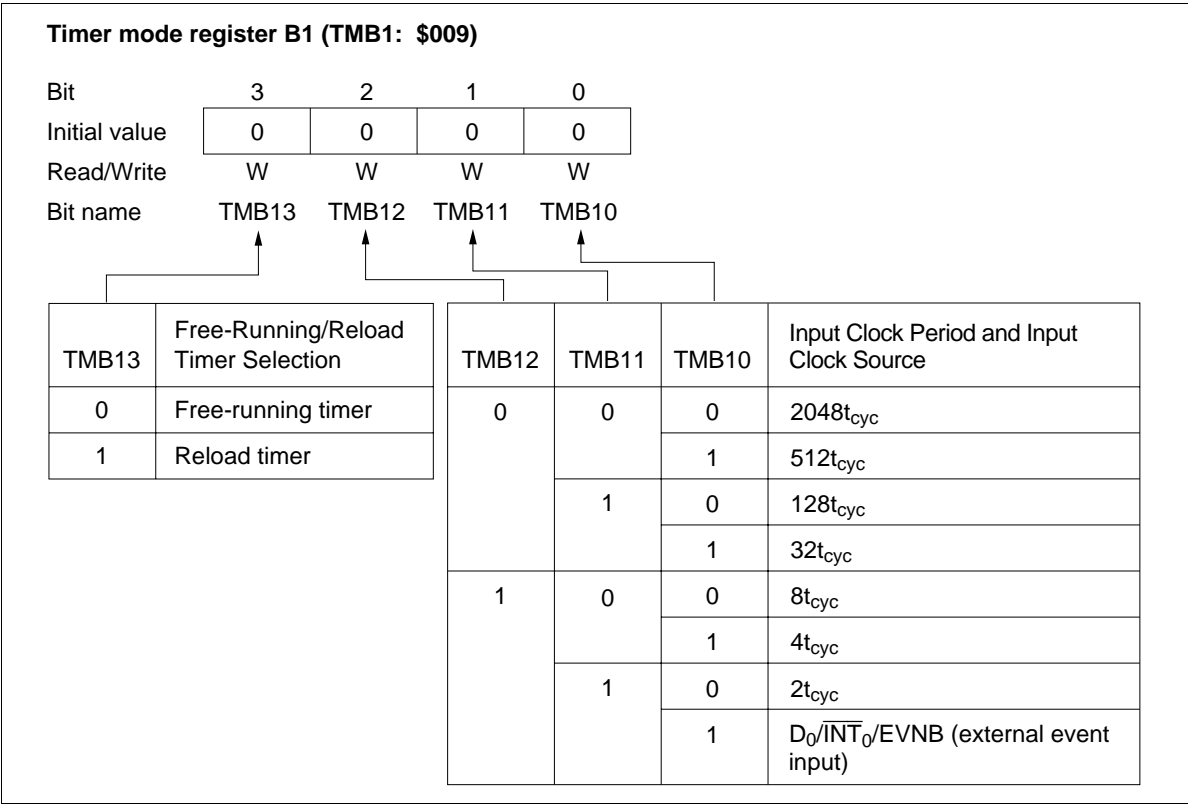
Figure 27 Timer Mode Register B1 (TMB1)
