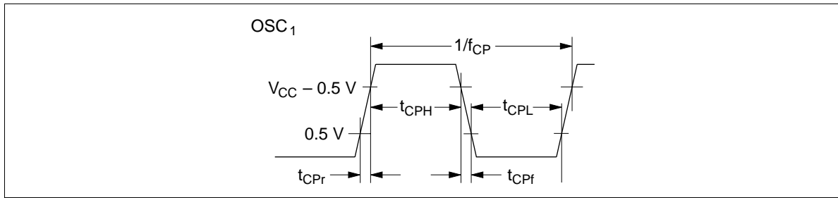
Figure 66 External Clock Timing
