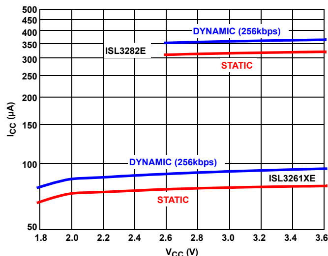
FIGURE 1. ISL3261XE REDUCES OPERATING I_{\text{CC}} BY A FACTOR OF 4 FROM PREVIOUS GENERATION RECEIVER ICs, AND OPERATES WITH SUPPLY VOLTAGES AS LOW AS 1.8V
