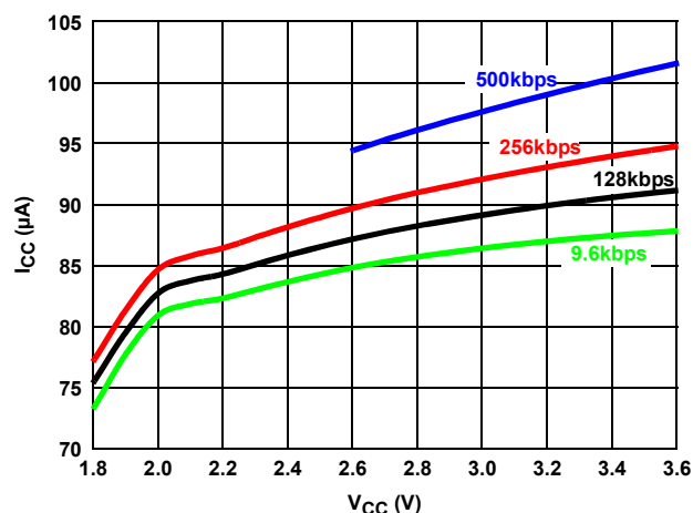
FIGURE 10. DYNAMIC SUPPLY CURRENT vs SUPPLY VOLTAGE AT DIFFERENT DATA RATES
