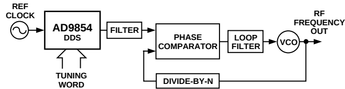
Figure 30. Agile High Frequency Synthesizer
