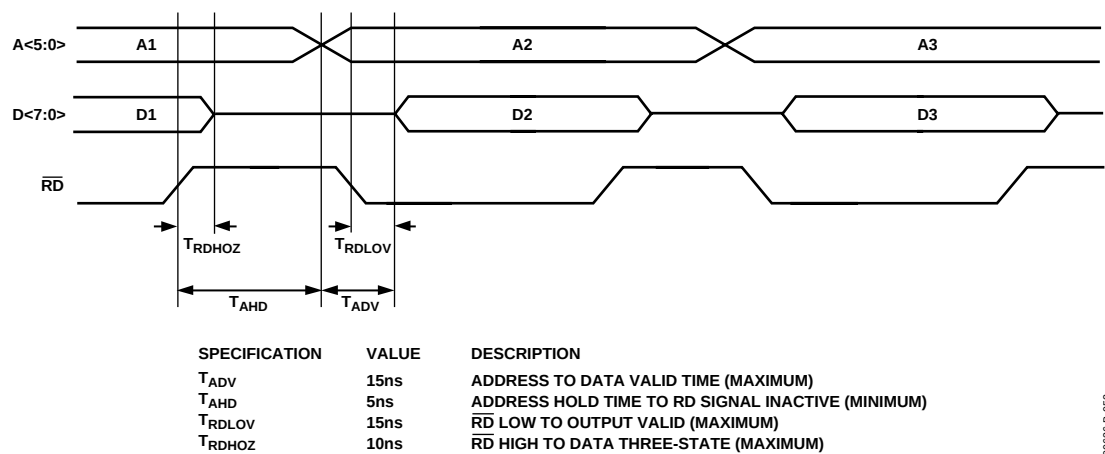
Figure 52. Parallel Port Read Timing Diagram
