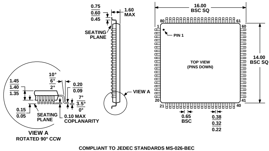
Figure 76. 80-Lead LQFP (ST-80-2) Dimensions shown in millimeters
