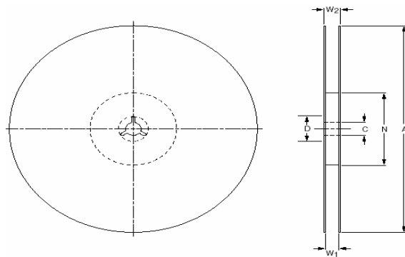
Fig.5 Reel
