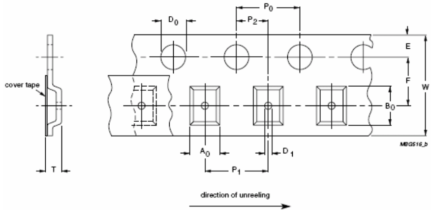
Fig.6 Embossed Dimensions
