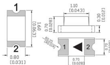
Package Outline Drawing:
