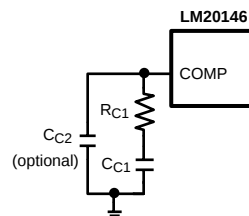
Figure 32. Compensation Network for LM20146
