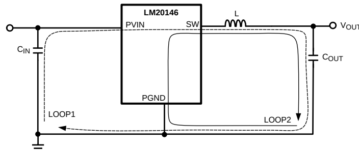
Figure 37. Schematic of LM20146 Highlighting Layout Sensitive Nodes
