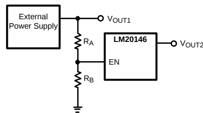
Figure 33. Sequencing LM20146 with Precision Enable
