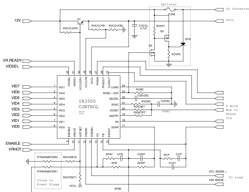
Figure 1 – Application Circuit
