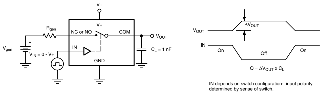
Figure 4. Charge Injection
