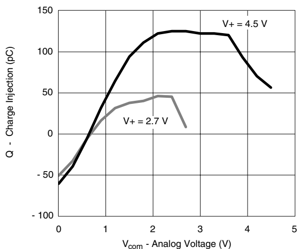
Charge Injection vs. Analog Voltage, DG2521
