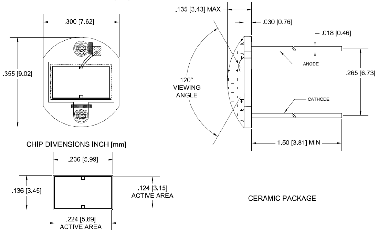
PACKAGE DIMENSIONS INCH [mm]
