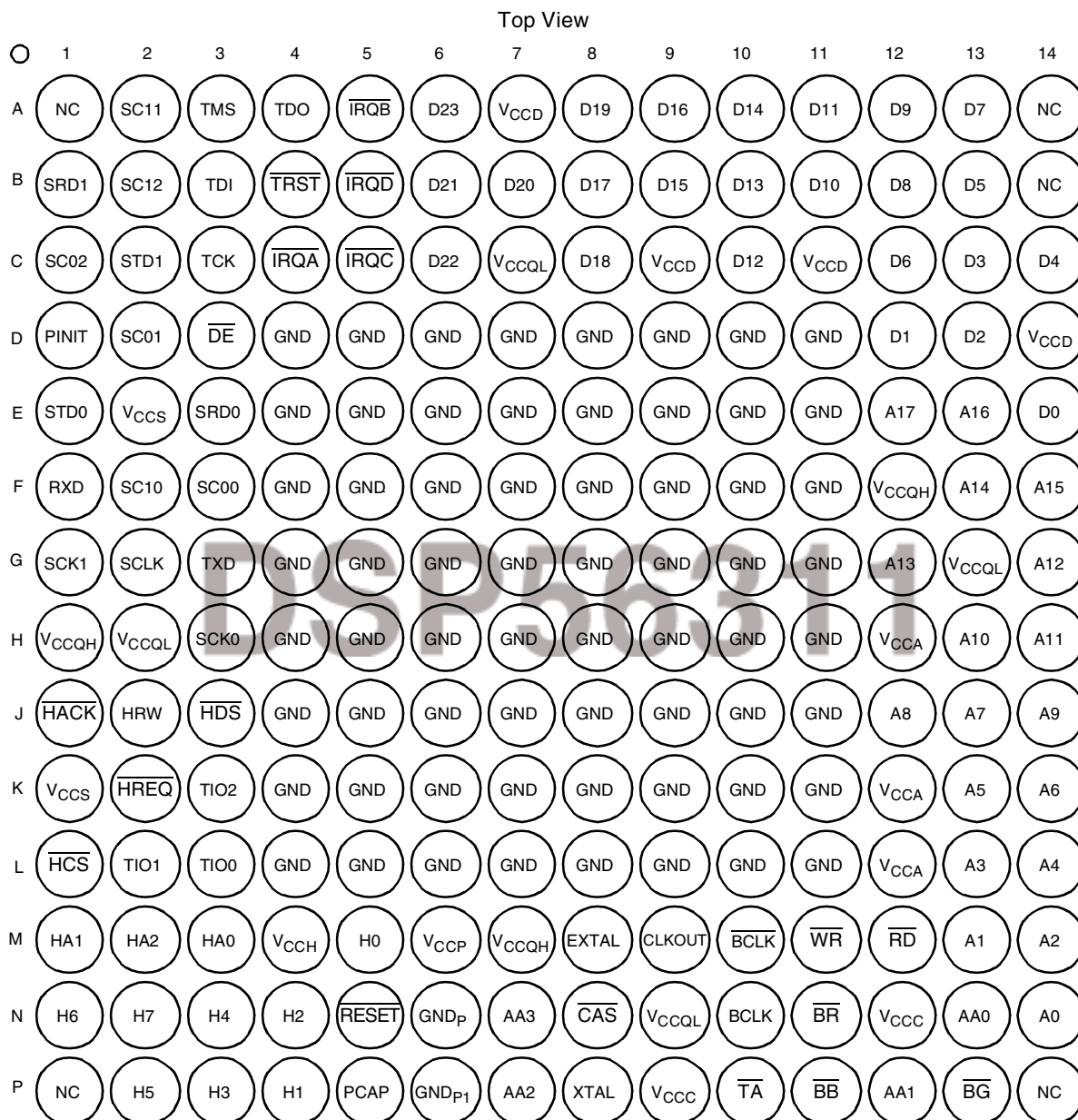
Figure 3-1. DSP56311 MAP-BGA Package, Top View
