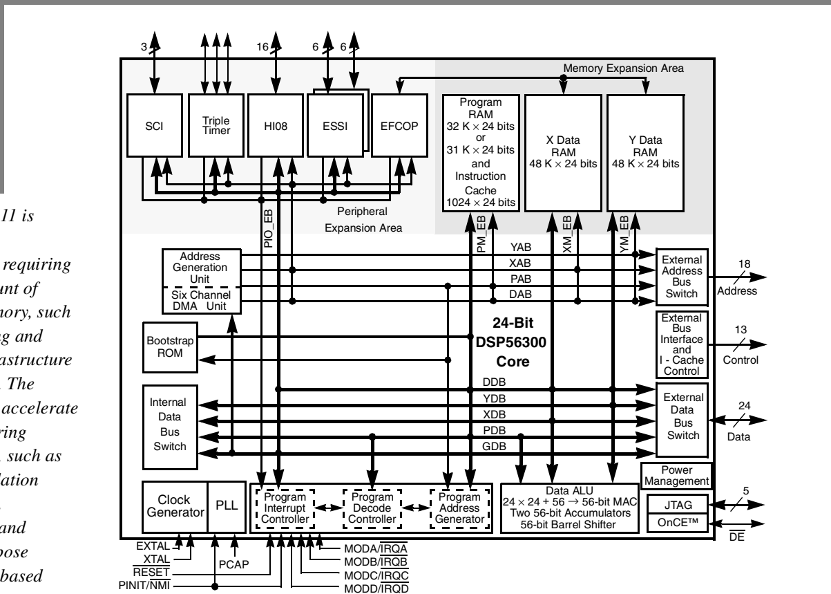
Figure 1. DSP56311 Block Diagram
