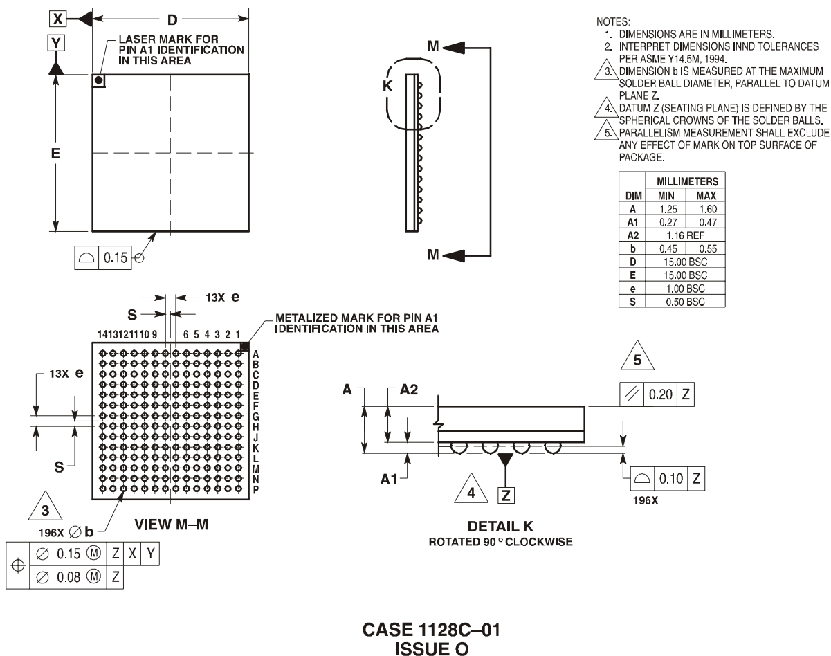
Figure 3-3. DSP56311 Mechanical Information, 196-pin MAP-BGA Package
