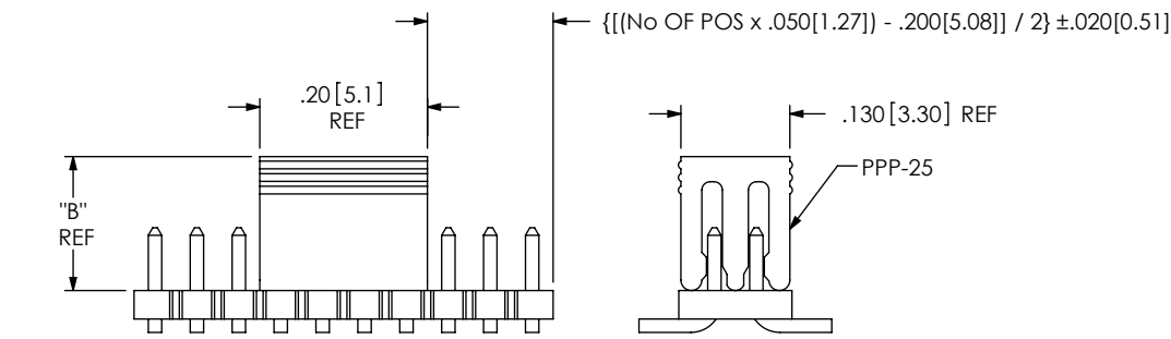
FIG 5 -DV-P OPTION FTS-110-02-XX-DV-P SHOWN (DIFFERENT AS SHOWN, OTHERWISE SAME AS FIG 1)
