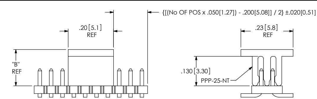
FIG 3 -DV-S OPTION (SEE NOTES 6 & 7) FTS-110-02-XX-DV-S SHOWN (DIFFERENT AS SHOWN, OTHERWISE SAME AS FIG 1) NOTE: 4 POSITIONS MUST BE ADDED TO PART CALLOUT TO ACHIEVE DIMS (NOT AVAILABLE WITH -A OPTION; ORDER -SA FOR ALIGNMENT PIN WITH SHROUD)
