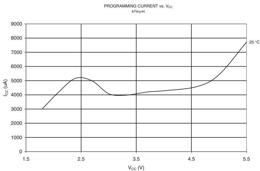
Figure 21-47. Programming Current vs. V_{CC} (ATtiny44)
