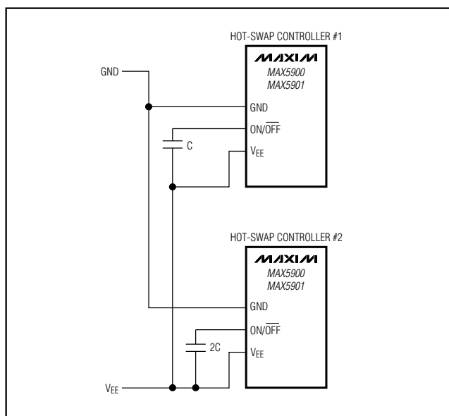
Figure 3. Power-Supply Sequencing
