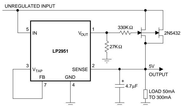
300mA REGULATOR WITH 0.75V DROPOUT
