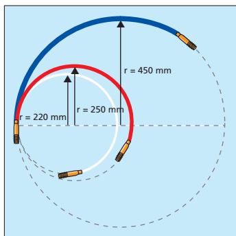
Overview on Rod Sets marginal bending radii.
