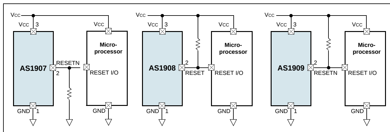
Figure 1. Application Diagrams
