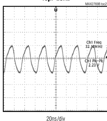
CLOCK OUTPUT DRIVER WITH 40pF LOAD
