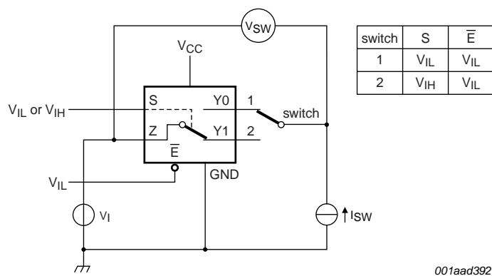
Fig 9. Test circuit for measuring ON resistance
