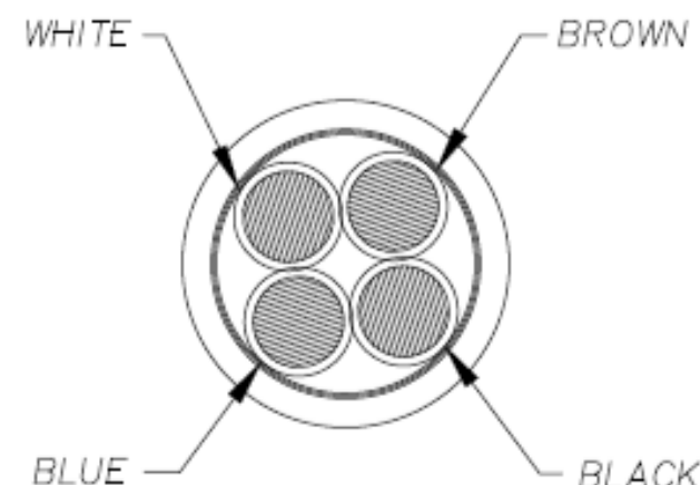
COLOR ROTATION OF CORD (FACE VIEW MALE)
