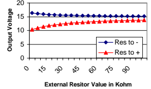
PM2012S15 Voltage Trim Adjust
