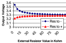
PM2012S03 Voltage Trim Adjust
