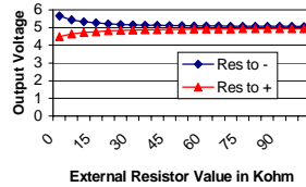
PM2012S05 Voltage Trim Adjust
