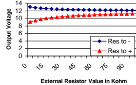
PM2012S12 Voltage Trim Adjust
