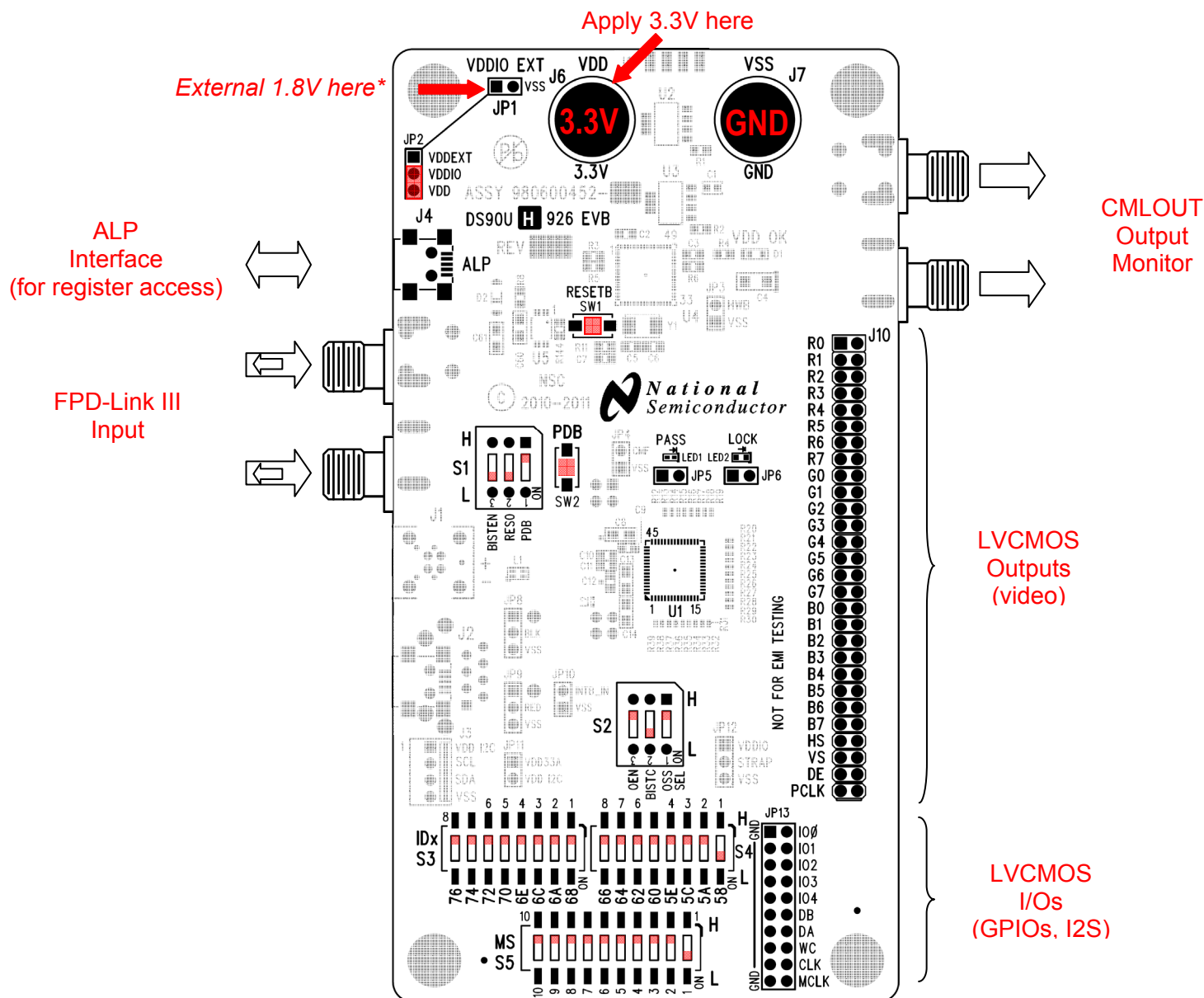
Figure 1: DS90UH926Q EVB
