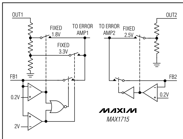
Figure 9. Feedback Mux
