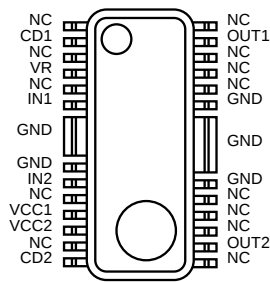
Fig.14 HSOP25
