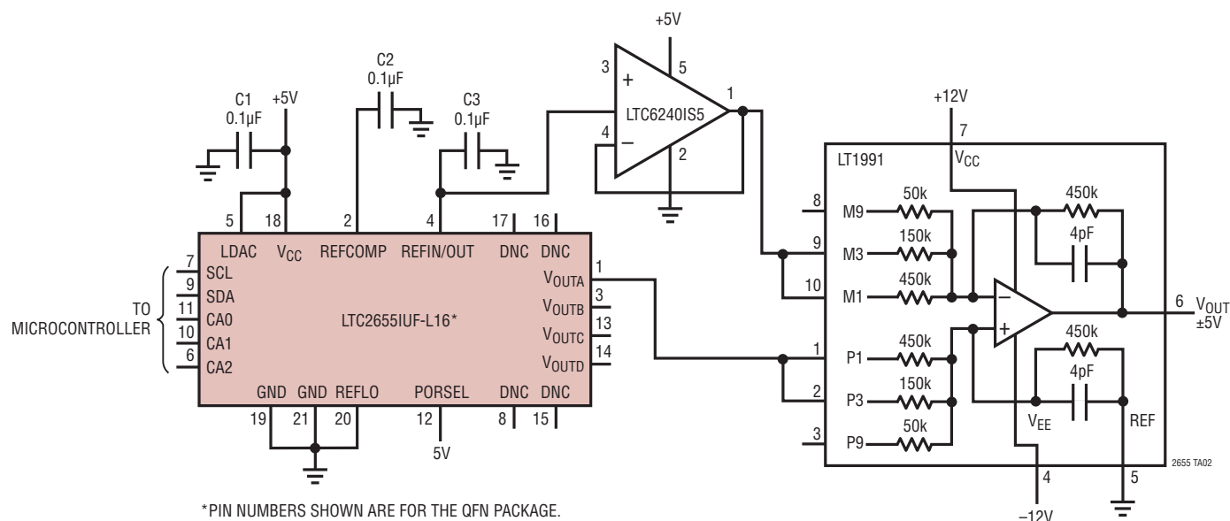
\pm 5V Bipolar Output DAC
