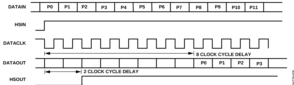
Figure 14. 4:4:4 Timing Mode
