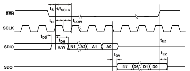
Figure 48. SPI 4-Wire Read Operation Timing
