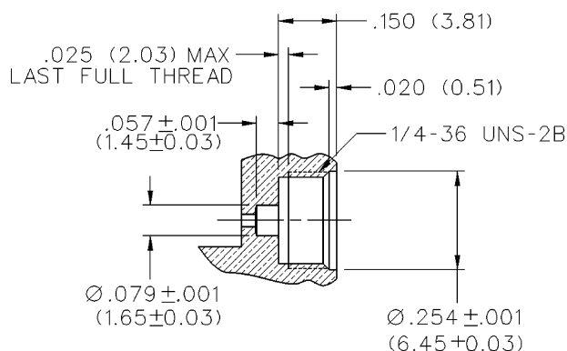
Mounting Hole Layout
