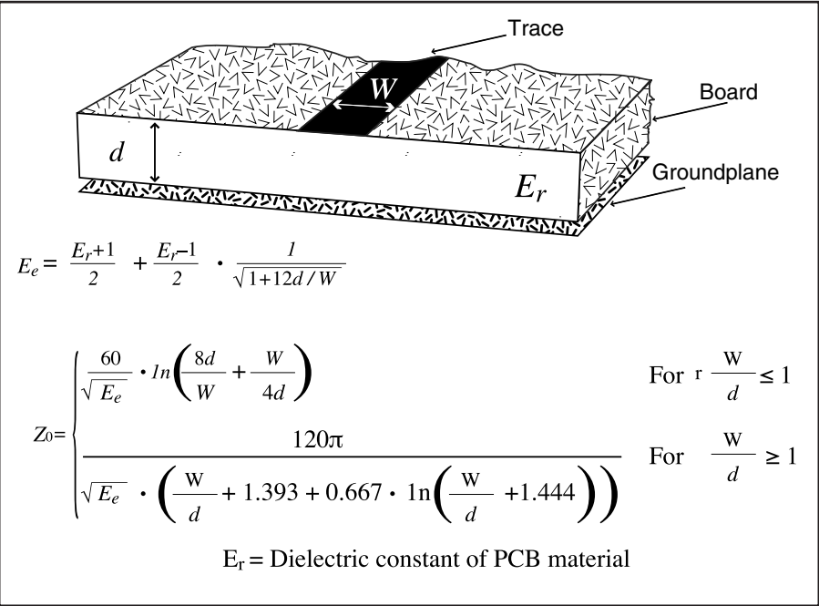
Figure 16: Microstrip Formulas ( E_r = dielectric constant of PC board material)
