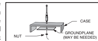
Figure 22: Remote Groundplane
