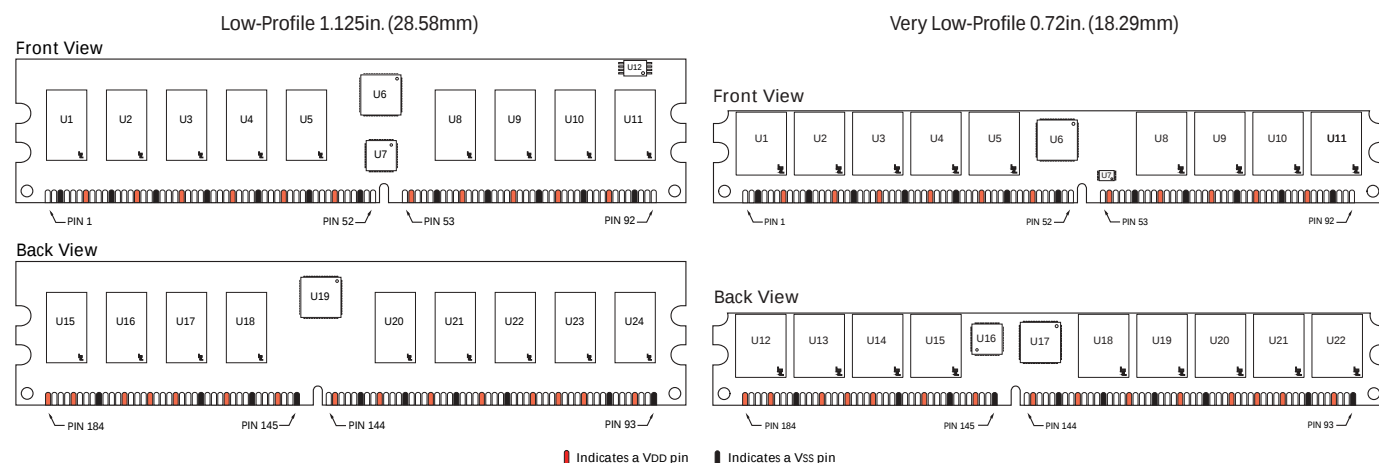
Figure 2: Pin Locations
