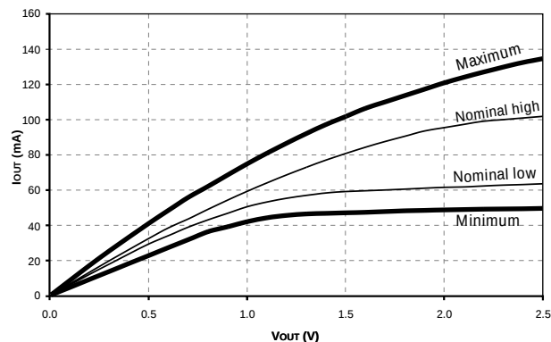
Figure 9: Pull-Up
