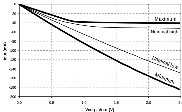
Figure 9: Pull-Up
