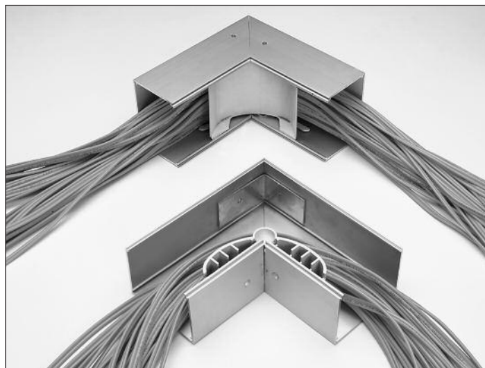
2" [51mm] Bend Radius Compliant Inserts installed in fittings.
