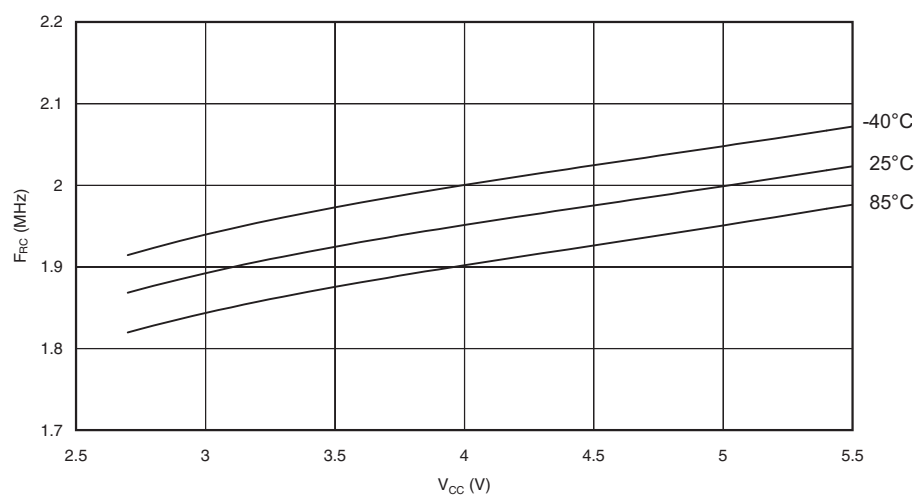
Figure 177. Calibrated 2MHz RC Oscillator Frequency vs. V_{CC}
