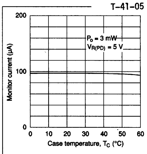
Figure 6 Temperature Dependence of Monitor Current
