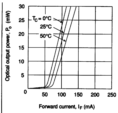
Figure 1 Optical Output Power vs. Forward Current
