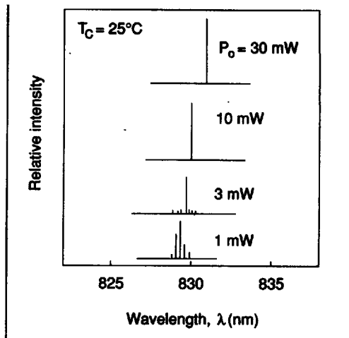
Figure 2 Lasing Spectrum
