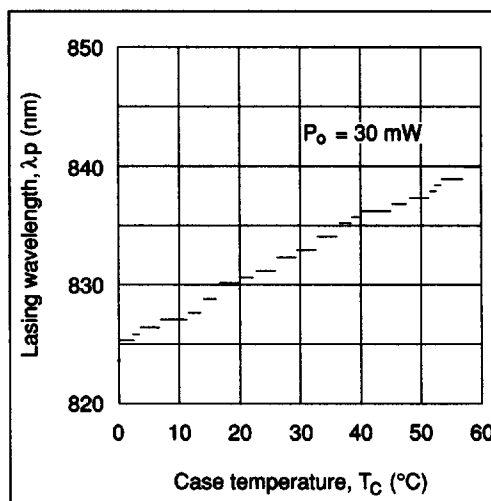
Figure 8 Temperature Dependence of Lasing Wavelength
